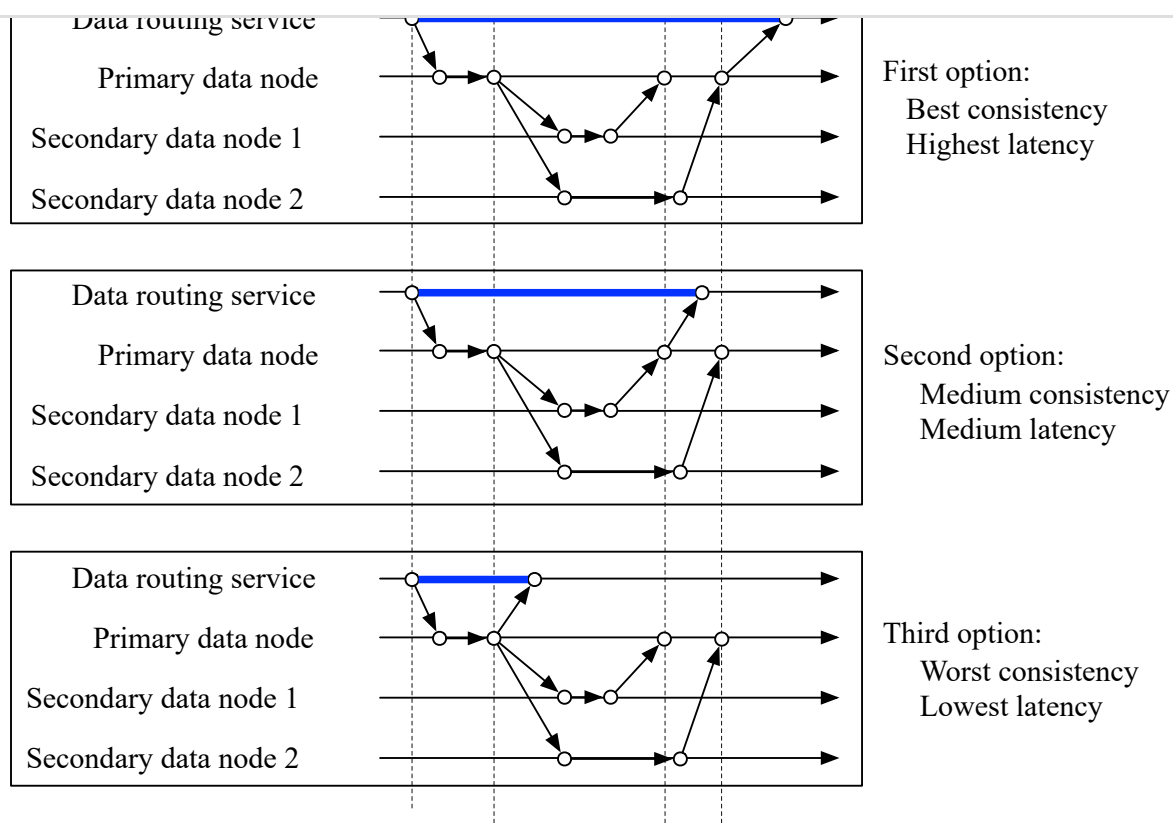
Figure 11 Trade-off between consistency and latency
